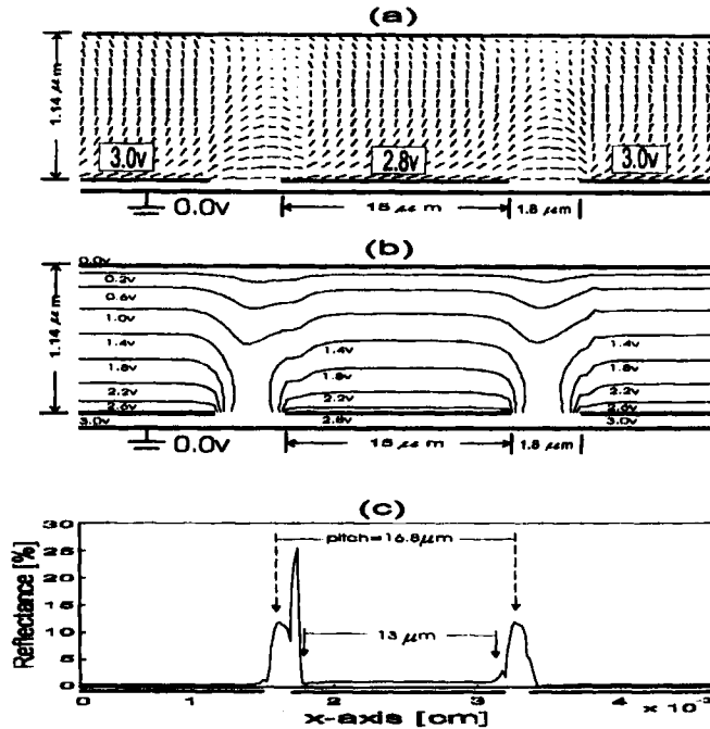
FIGURE 6 (a) The LC directors driven by the frame inversion method. (b) Calculated equal potential contours. (c) 2-D reflectance profile exhibits that the fringe field effect is quite different between the dot and frame inversion methods.
