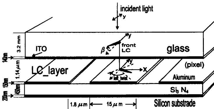
FIGURE 4 The 2-D MTN-90° cells used to calculate the distribution of the nematic director orientation and the reflectance. The front LC director is set at an angle \beta of 20° to the polarization state ( y -axis) of the incident light.
