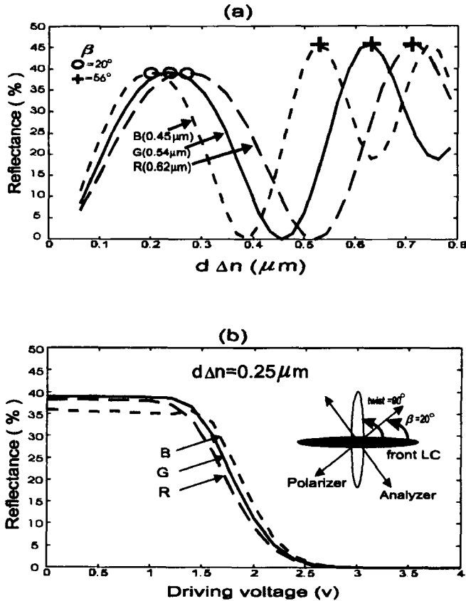
FIGURE 1 (a) The maximum reflectance as a function of d\Delta n of MTN- 90^\circ cells at R, G, and B incident wavelengths. (b) Reflectance as a function of driving voltage at d\Delta n = 0.25 \mu\text{m} and \beta = 20^\circ .
